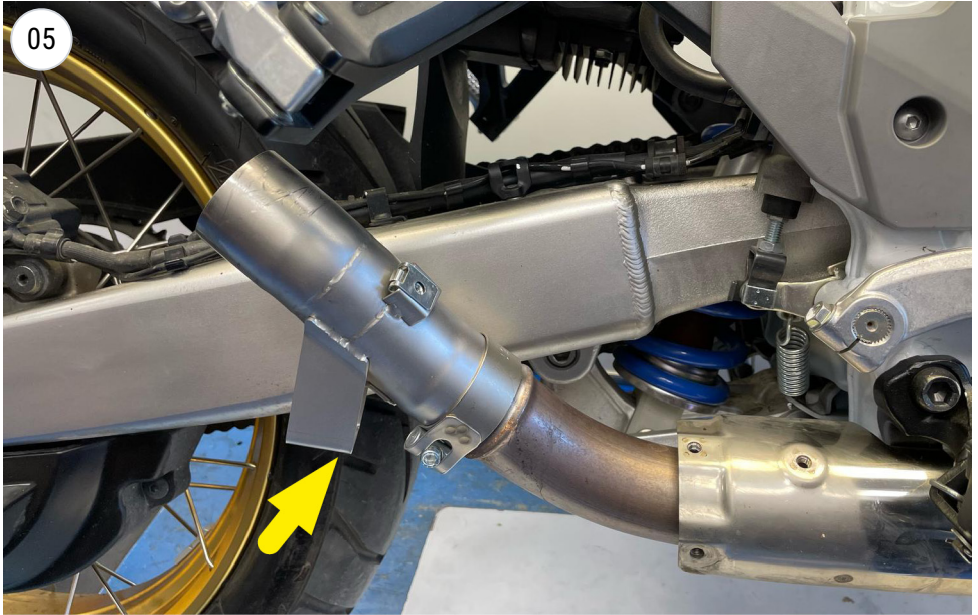
install the pipe with the clamp
