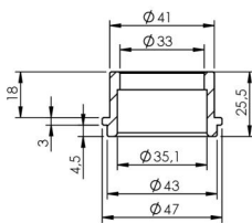
S.S. Bushing P/N 204833R
