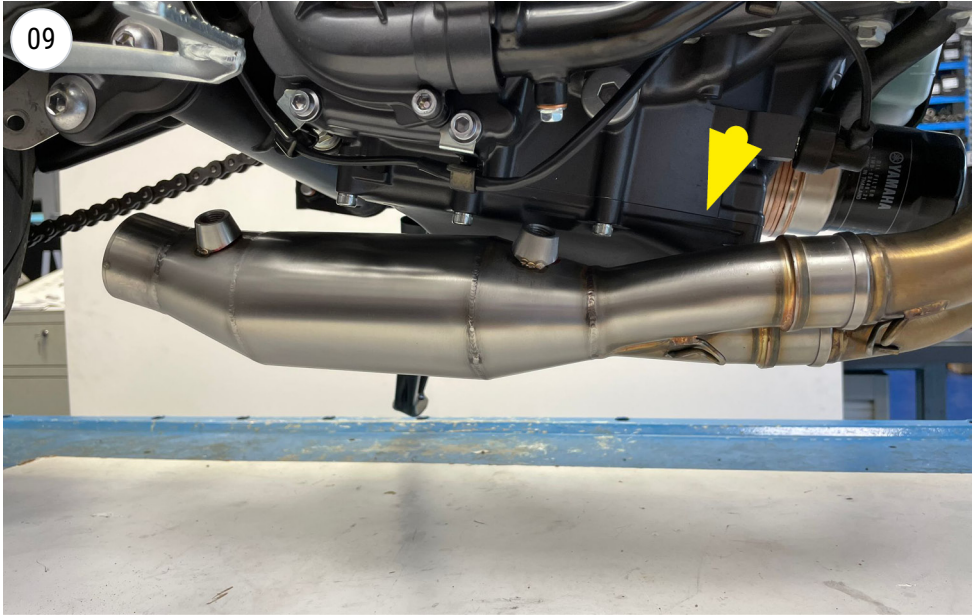
fit the secondary pipe
