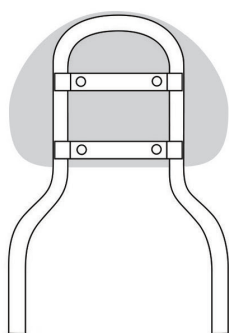
Hole pattern A Universal bar with 2 brackets
